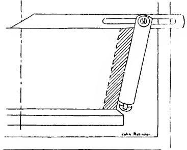
FIG. 278. SETTING T-BEVEL FROM DRAWING.
